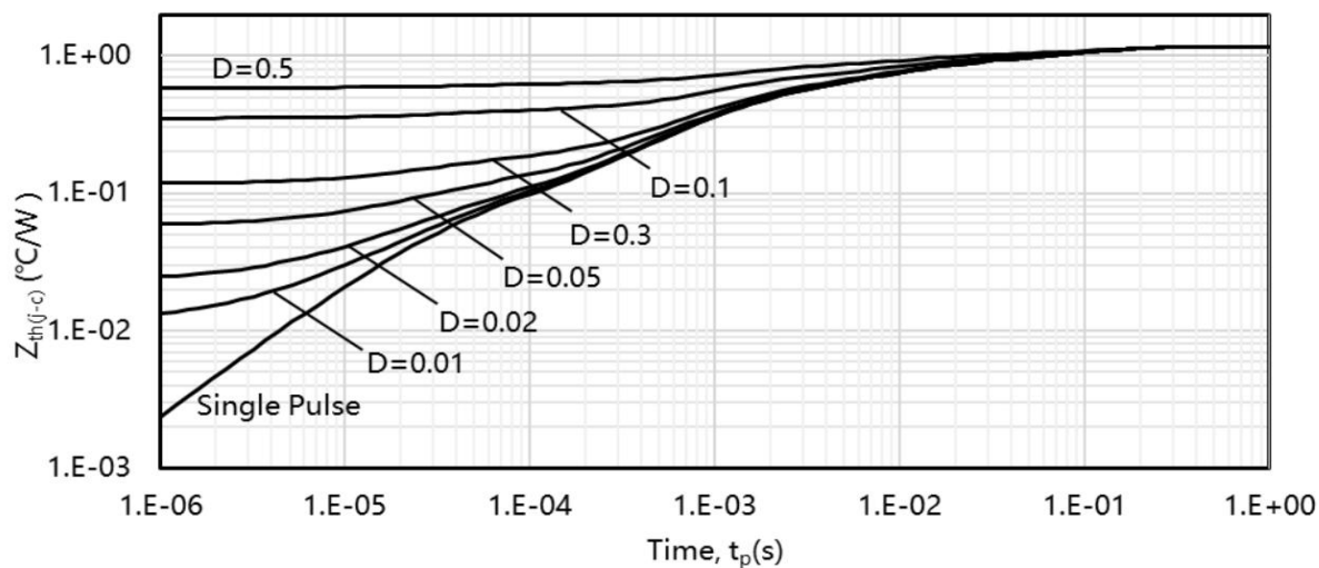
Figure 7. Max. transient thermal impedance, Z_{th(j-c)} = f(t_p) , parameter: D = t_p/T
