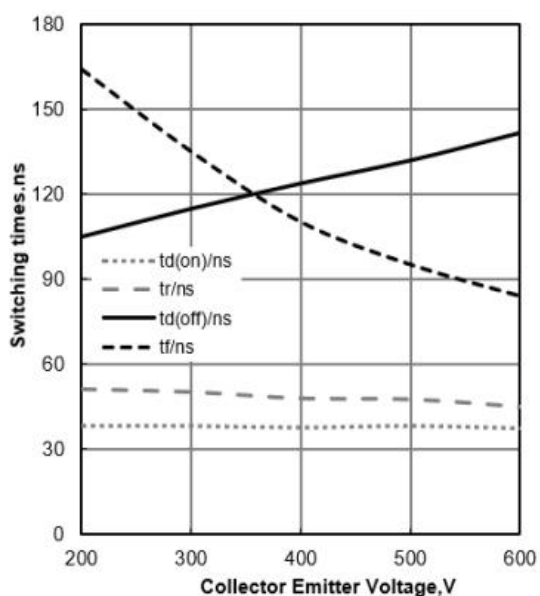
Figure 15: Typical Switching Times vs. VCE ( T_J=25^{\circ}\text{C} , V_{GE}=15\text{V} , I_c=60\text{A} , R_g=5\Omega )
