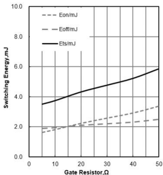
Figure 10: Typical Switching Energy vs. Gate Resistor ( T_J=25^{\circ}\text{C} , V_{CE}=400\text{V} , V_{GE}=15\text{V} , I_C=60\text{A} )
