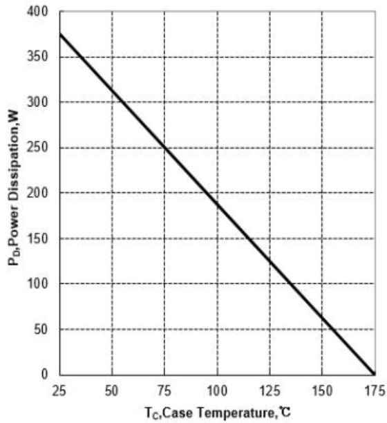
Figure 1: Power Dissipation
