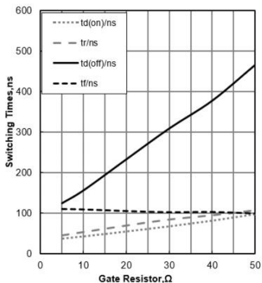
Figure 9: Typical Switching Times vs. Gate Resistor ( T_J=25^{\circ}\text{C} , V_{CE}=400\text{V} , V_{GE}=15\text{V} , I_C=60\text{A} )
