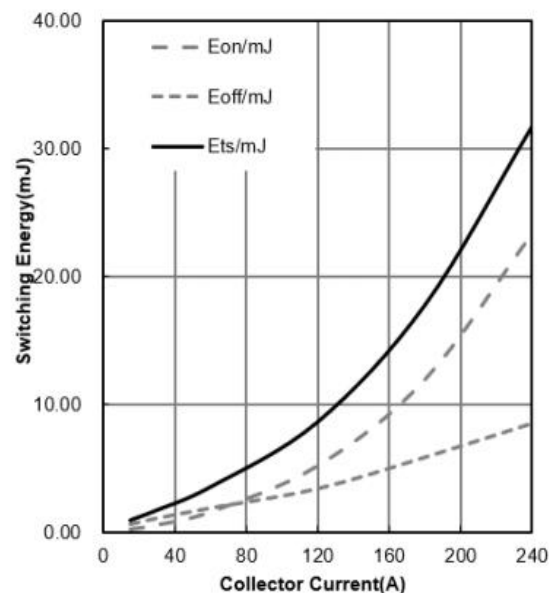
Figure 14: Typical Switching Energy vs. Collector Current ( T_J=25^{\circ}\text{C} , V_{CE}=400\text{V} , V_{GE}=15\text{V} , R_g=5\Omega )
