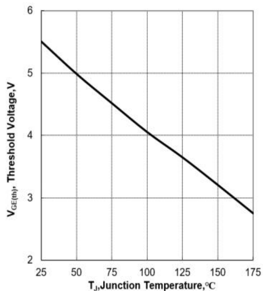
Figure 8: Typical Gate-Emitter Threshold Voltage vs. Junction Temperature
