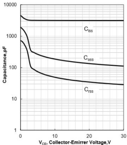
Figure 17: Typical Capacitance vs. Collector- Emitter Voltage
