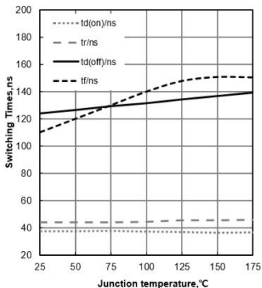
Figure 11: Typical Switching Times vs. Junction Temperature ( V_{CE}=400\text{V} , V_{GE}=15\text{V} , I_C=60\text{A} , R_g=5\Omega )
