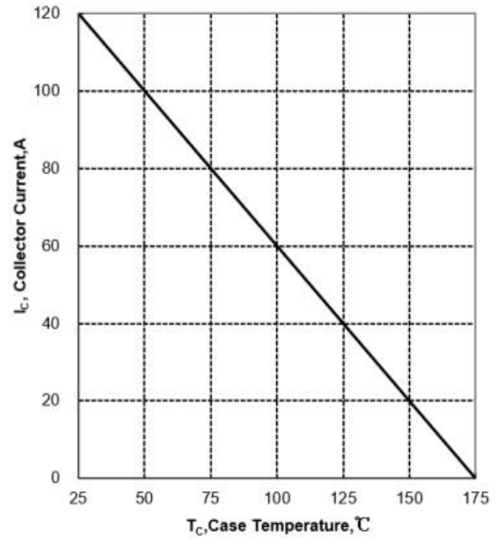
Figure 2: Collector Current vs. Case Temperature
