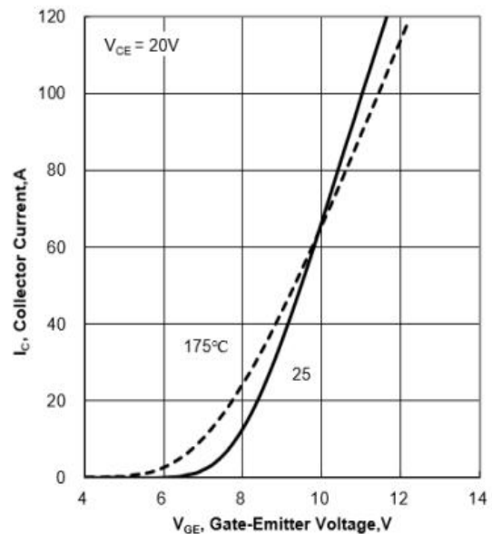
Figure 4: Typical Transfer Characteristics
