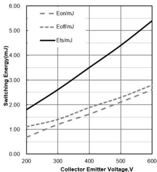
Figure 16: Typical Switching Energy vs. VCE ( T_J=25^{\circ}\text{C} , V_{GE}=15\text{V} , I_c=60\text{A} , R_g=5\Omega )
