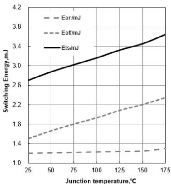
Figure 12: Typical Switching Energy vs. Junction Temperature ( V_{CE}=400\text{V} , V_{GE}=15\text{V} , I_C=60\text{A} , R_g=5\Omega )
