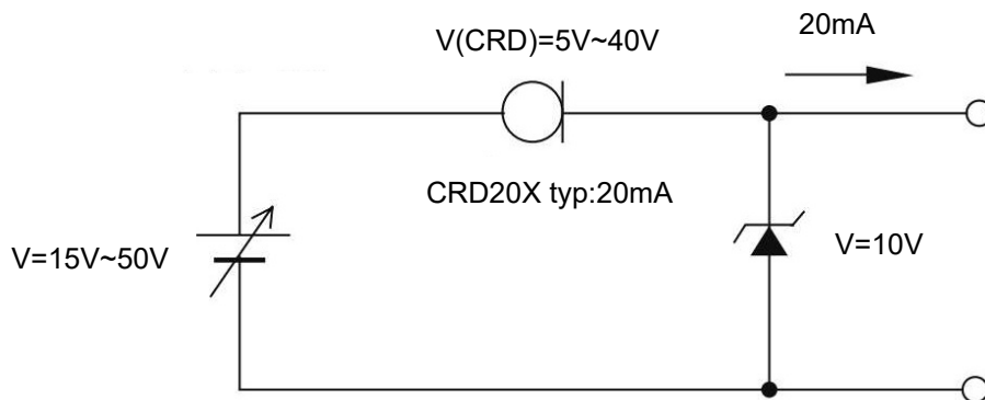
(1) Combination of Zener diode and CRD
