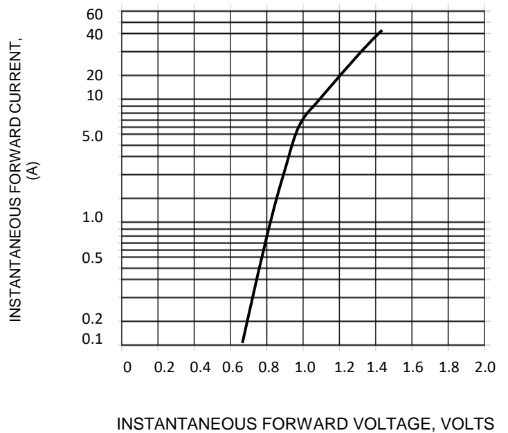
FIG.4-TYPICAL FORWARD CHARACTERISTICS
