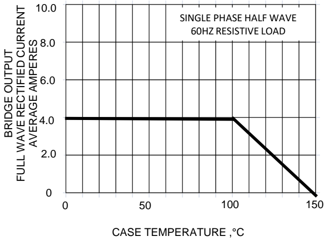
FIG.1-DERATING CURVE FOR OUTPUT RECTIFIED
