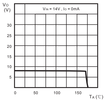
Thermal Shutdown
