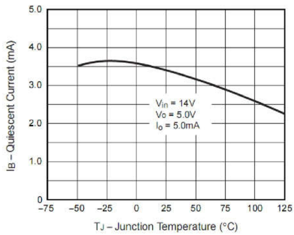
Figure.10 Quiescent Current vs. Junction Temperature
