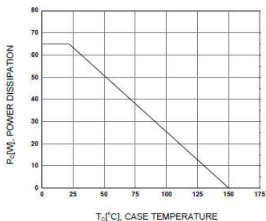
Figure 5. Power Derating
