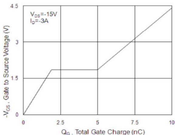
Fig.4 Gate-charge Characteristics
